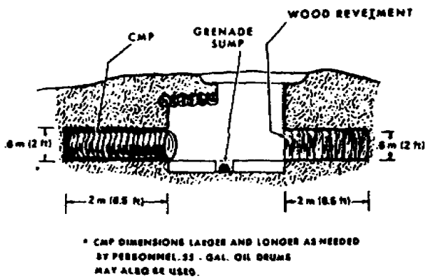
Figure 1-13. Two-man foxhole with offset constructed of timber and culvert.
